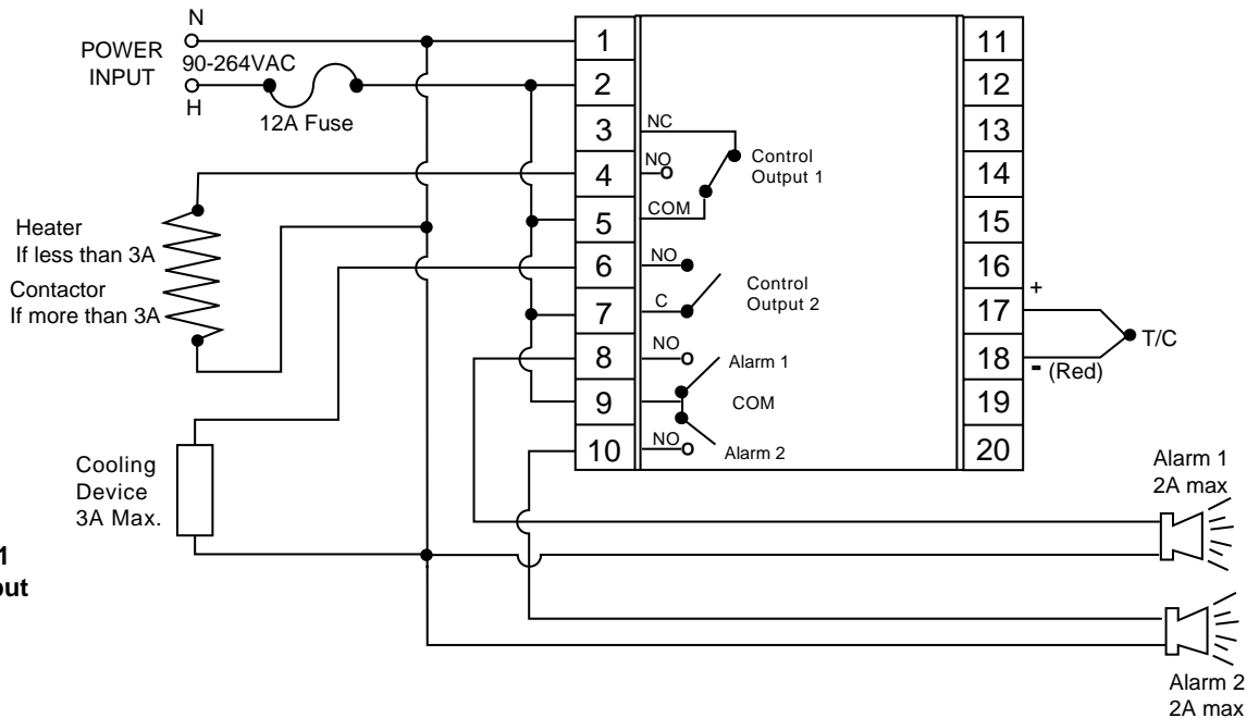
ETR-4130-313221 Thermocouple Input 3-32VDC Output 1 Relay Output 2 Dual Alarms
