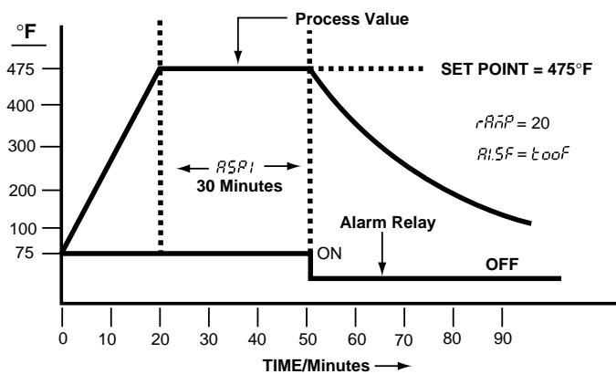
Diagram 1: Ramp and Soak
