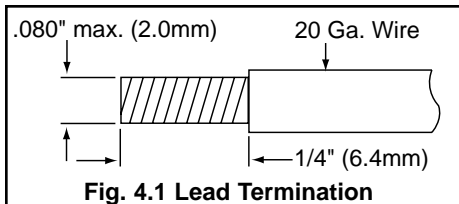
Fig. 4.1 Lead Termination
