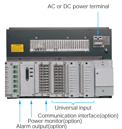
Rear panel of the stand-alone model
