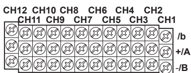
Input terminal block of the DX1012 and DX1012N
